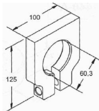
MANCAL PINO TENSOR TRUCK / CARRETA GUERRA Ø 60,3MM
