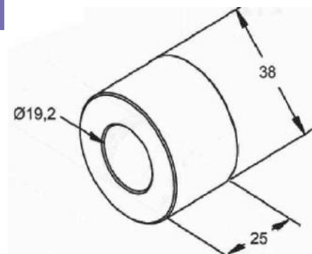
ROLDANA DO PATIM TRUCK / CARRETA RANDON 72 Á 78 (38 X 19,2 X 25)
