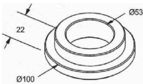
MANCAL EXTERNO NOMA 53 X 100 X 22
