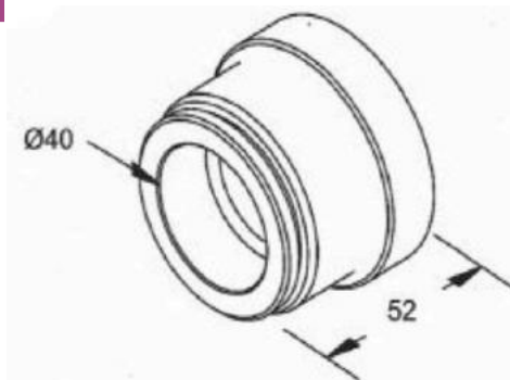
GUIA INFERIOR DO ENGATE RANDON
