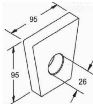
MANCAL DO PINO TENSOR RANDON FURO Ø26MM
