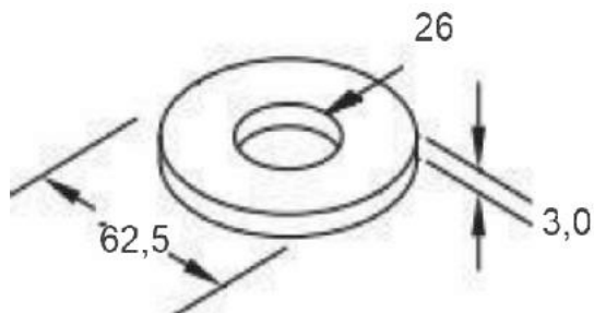
ARRUELA INTERNA PINO TENSOR TODOS 62,5 X 26,0 X 3,0MM
