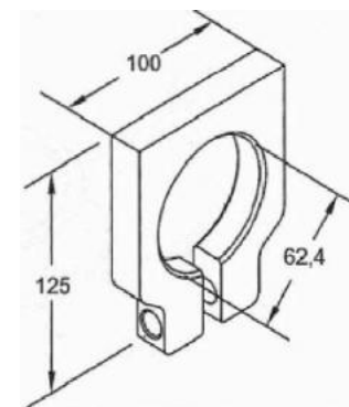
MANCAL EXT. DO PINO TENSOR TRUCK / CARRETA RODOVIÁRIA Ø 62,4MM
