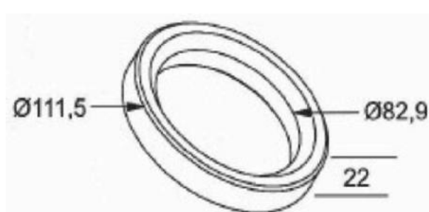
ANEL PISTA TRUCK RANDOM
