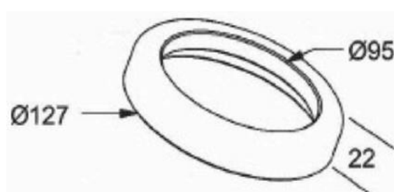
ANEL PISTA RANDOM MASTER 127 X 95 X 22
