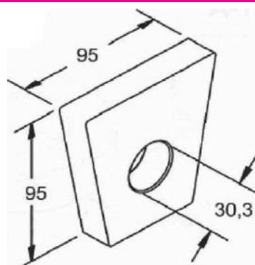
MANCAL PINO TENSOR TRUCK / CARRETA GUERRA FURO Ø30,3MM
